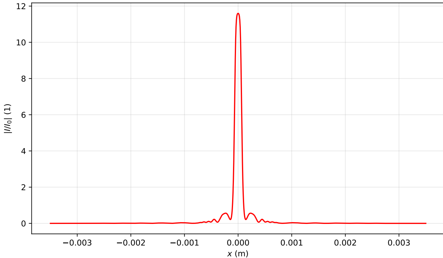
Intensity profile I(x, y = 0, z = 0.318)/I_0 , P_{in}=6.0P_{cr} , artificial time
